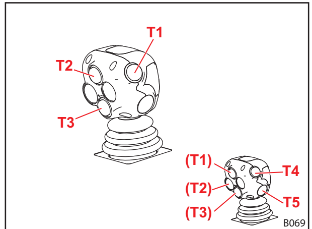
Abb. 76 STOLL Trac Control (3 Taster)
