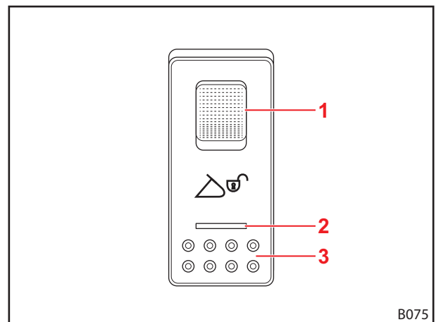
Abb. 80 Hydro-Lock-Schalter
