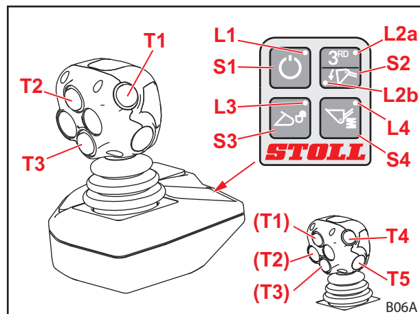
Σχ. 66 STOLL Pro Control
